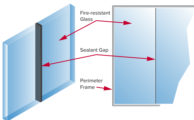
Figure 10 – Example of fire-resistant butt-joint system
