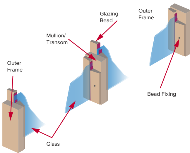
Figure 2b – Vertical section through glazed timber screen
